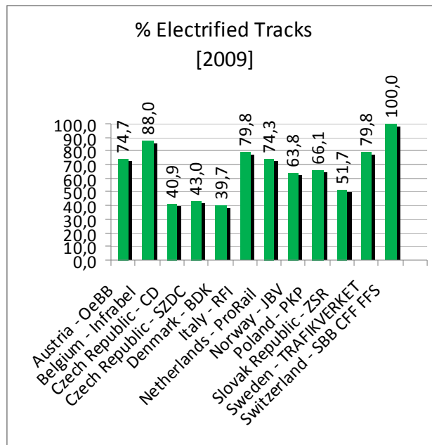
Figure 2 – Percentage electrified lines of mid-size railway networks in Europe 2009
