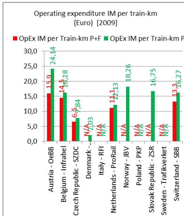
Figure 17 – Operating expenditure of infrastructure manager per train-km in mid-size railway networks in Europe 2009
