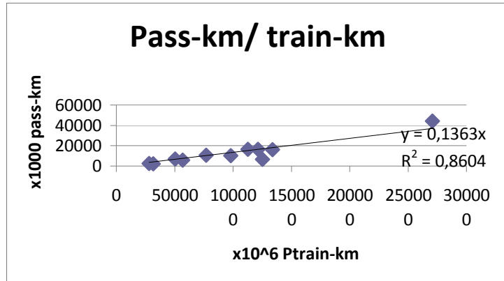
Figure 9 – Scatter diagram of passenger-km per train-km of incumbent operator in mid-size European railway networks 2009
