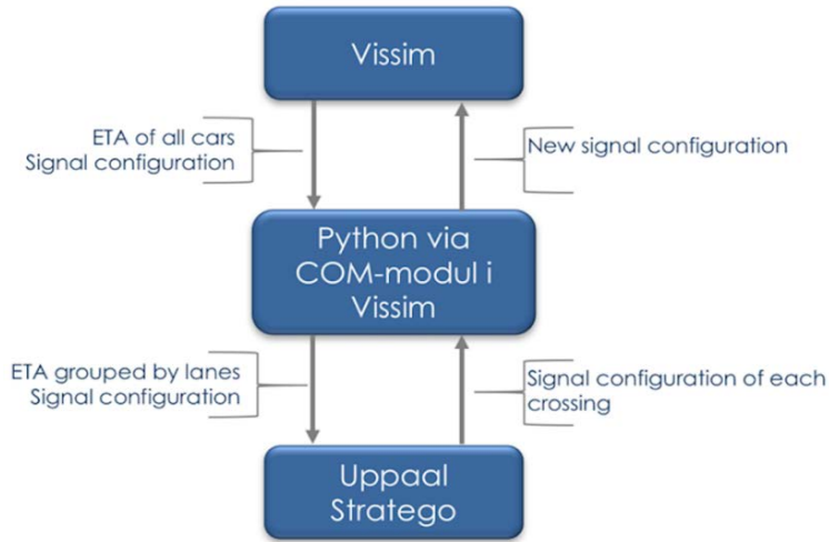
Figure 2 - The communication between Vissim, Python and Uppaal Stratego.
