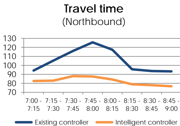
Figure 110 – The north bound travel time
