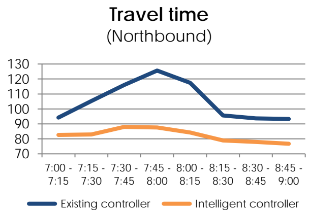
Figure 10 – The north bound travel time
