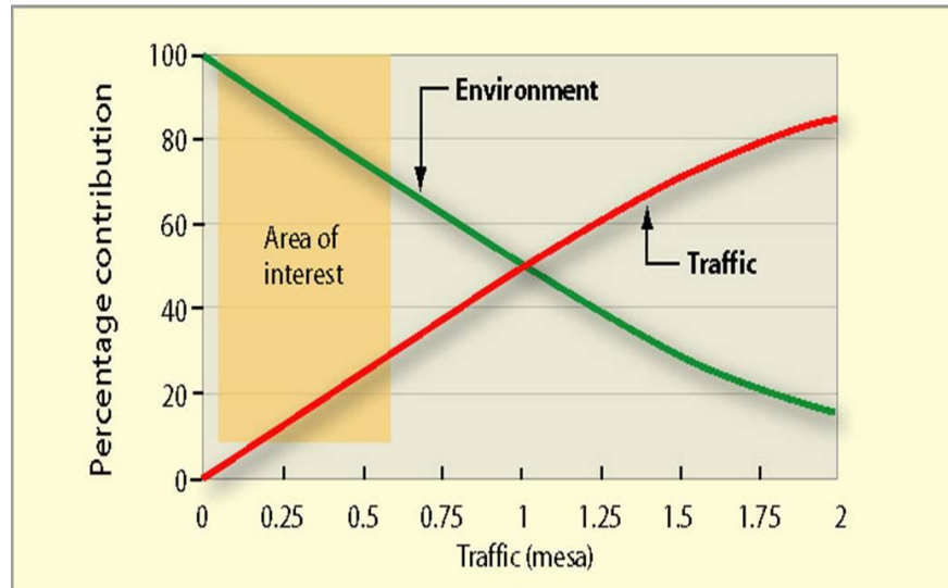
Figure 4 The relatively higher component impact of pavement environment
