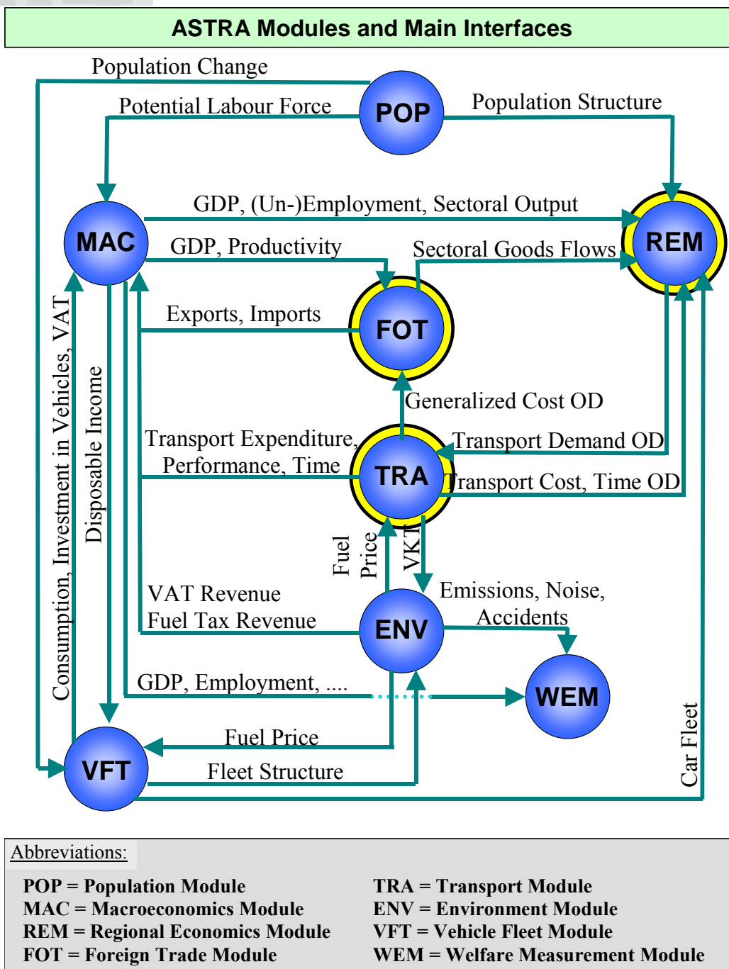
Figure 1: Overview on the ASTRA model
